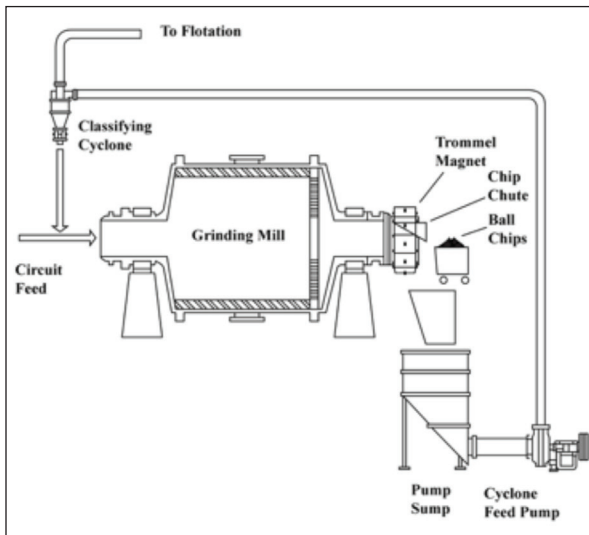
Figure 3: Trunnion magnet replaces the trommel screen
