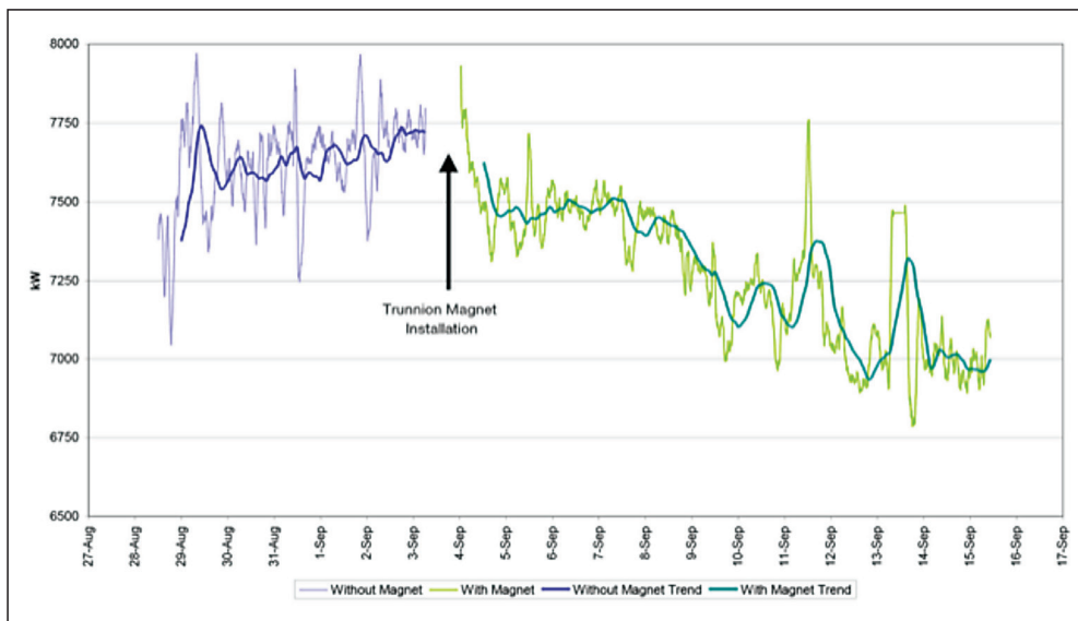
Figure 6: Ball Mill Total kW Before and After Trunnion Magnet
