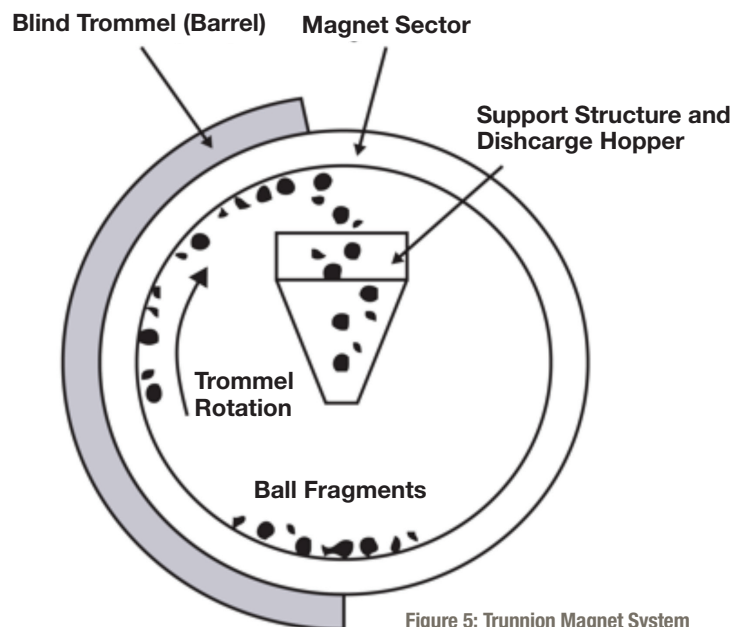
Figure 5: Trunnion Magnet System
