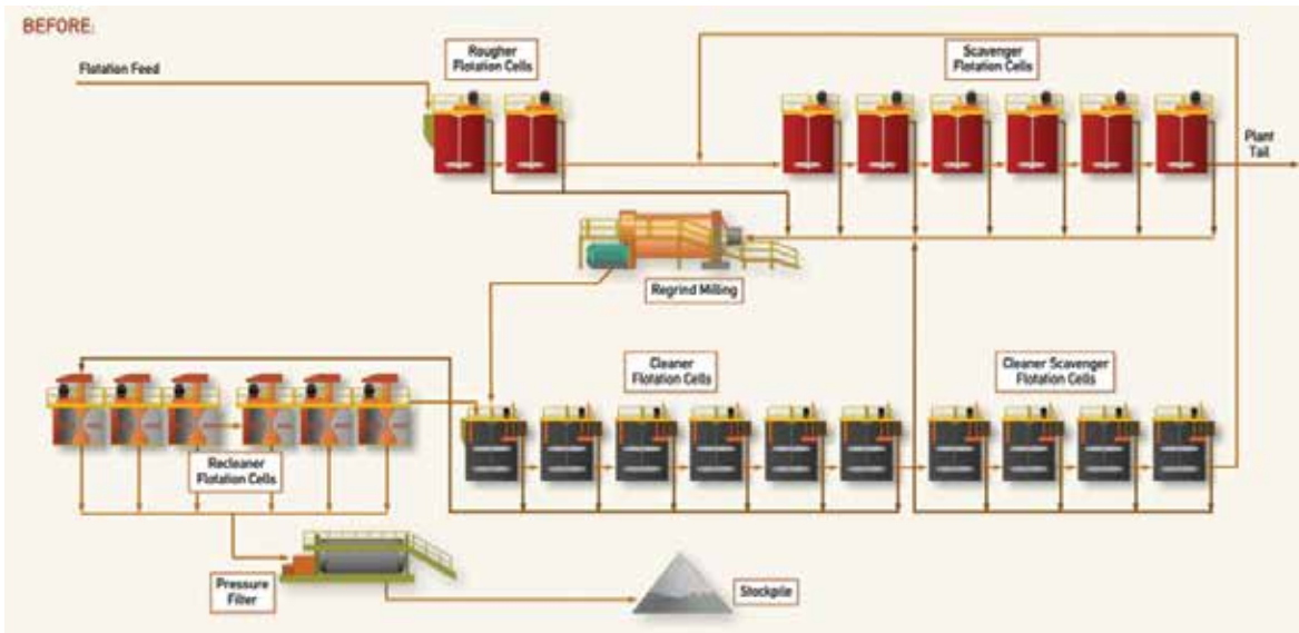
FIGURE 1 DeGrussa copper mine processing flow sheet, 2014
