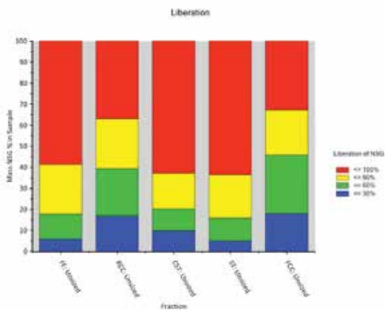
FIGURE 3 Non sulphide gangue liberation in float feed (FF), recleaner concentrate (RCC), cleaner scavenger tail (CST), scavenger tail (ST), flash cleaner concentrate (FCC)
