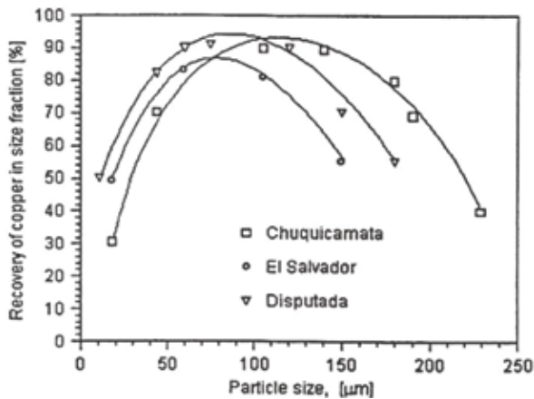
FIGURE 4 Copper recovery at various size fractions (%)
