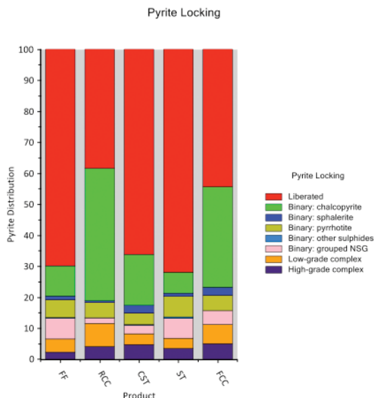
FIGURE 2 Pyrite liberation in float feed (FF), recleaner concentrate (RCC), cleaner scavenger tail (CST), scavenger tail (ST), flash cleaner concentrate (FCC)
